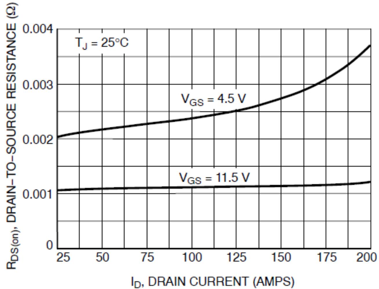
Figure 4. On-Resistance vs. Drain Current and Gate Voltage
