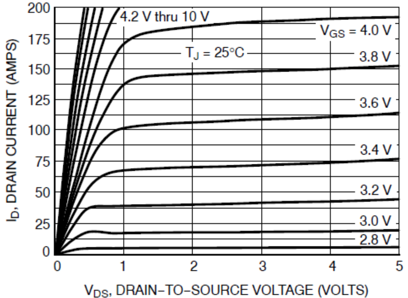
Figure 1. On-Region Characteristics
